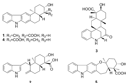
Figure 1. Structures of bacterial indolosesquiterpenes, xiamycin ( 1 ), indospene ( 2 ), sespenine ( 3 ), oridamycin ( 4 ), and oxiamycin ( 5 ).
